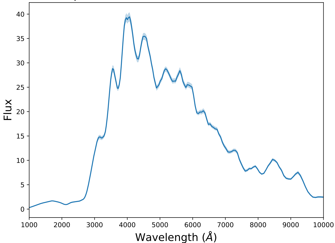
Spectrum 3 for transient SNIax at z=0.41
